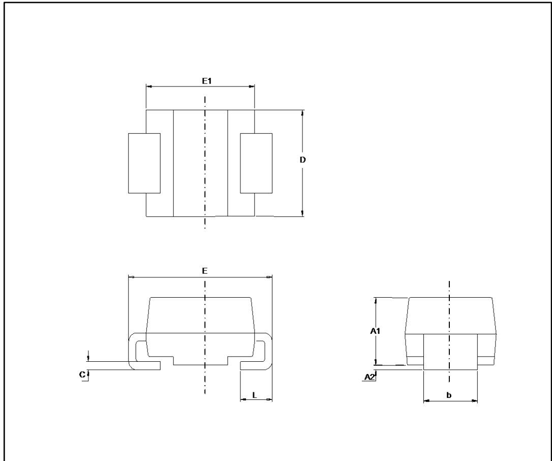
Figure 10: SMB package outline
