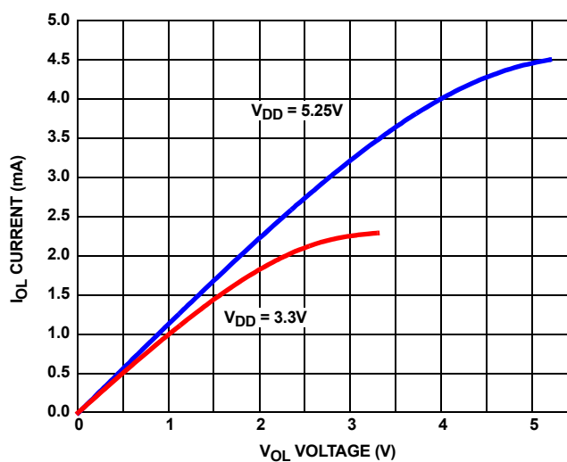
FIGURE 20. I_{OL} vs V_{OL} vs V_{DD} for \overline{\text{INT}} and \overline{\text{ALM}}
