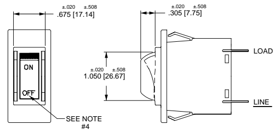
ROCKERGUARD CONFIGURATION
