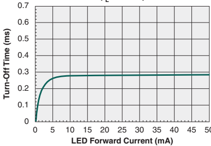
Typical Turn-Off Time vs. LED Forward Current (I L =80mA)
