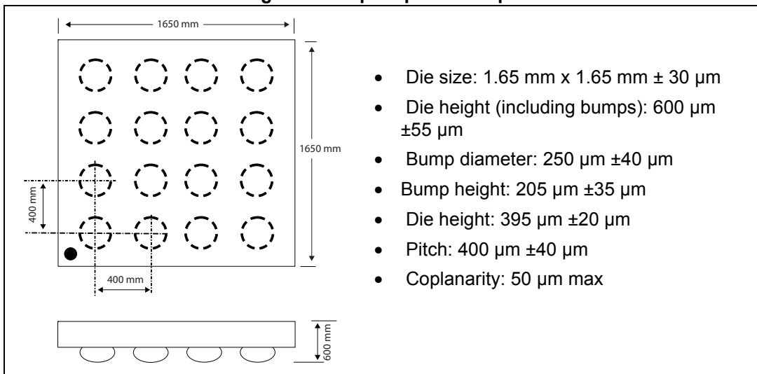
Figure 78. Flip-chip - 16 bumps
