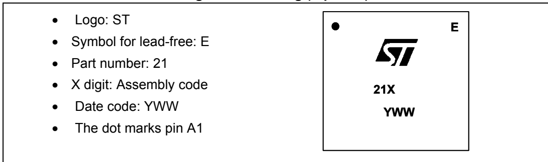
Figure 78. Flip-chip - 16 bumps
