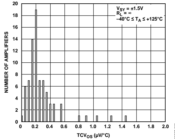
Figure 15. TCV_{OS} Distribution, SOT-23
