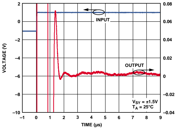
Figure 30. Settling Time
