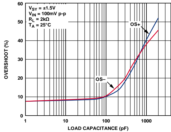
Figure 32. Overshoot vs. Load Capacitance
