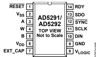
Figure 5. Pin Configuration
