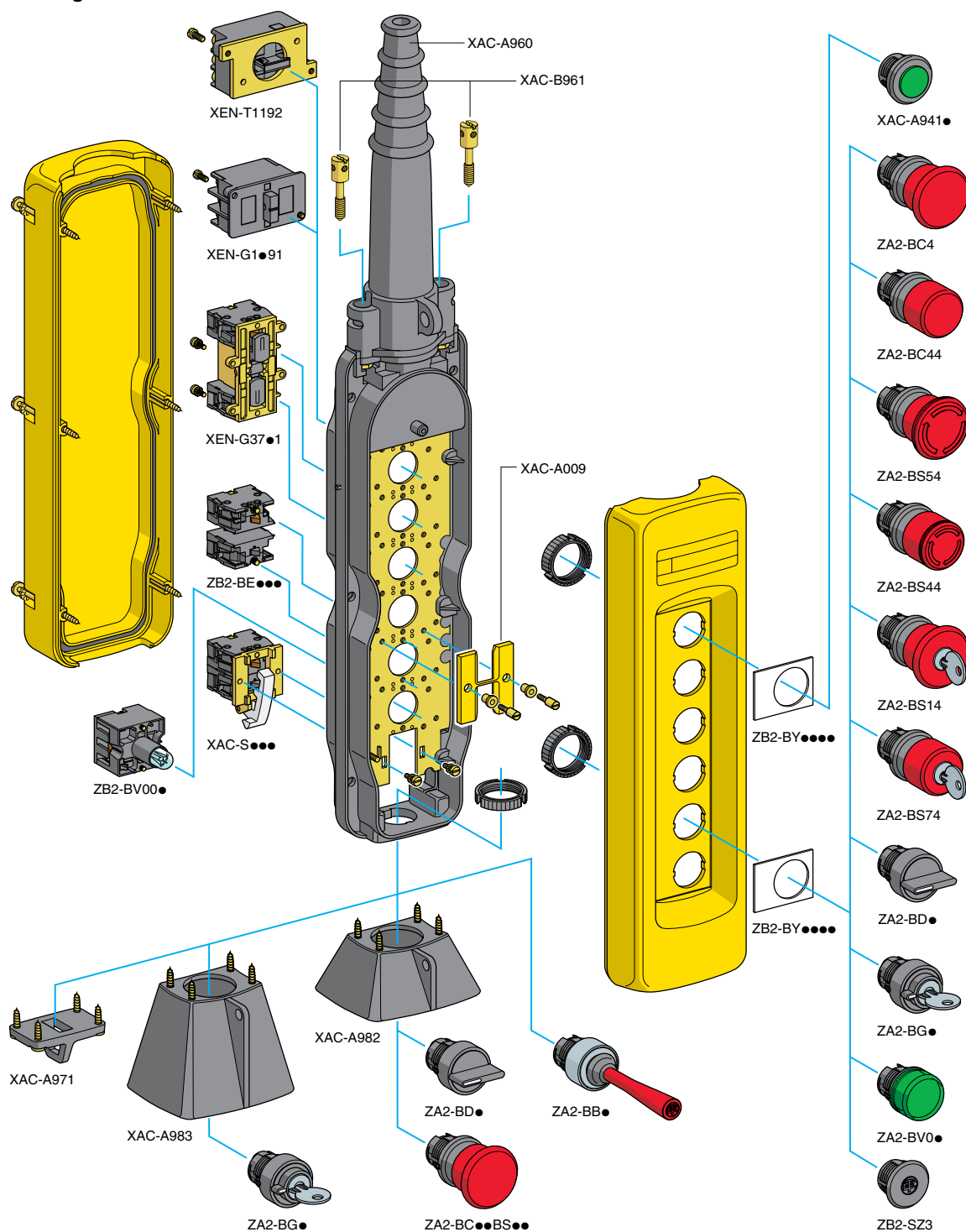
Exploded Drawing
