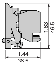
Plug-in connector ZB4BZ10•4, BZ1414
