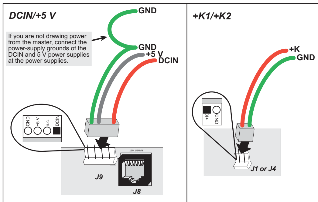
Figure 5. Power-Supply Connections
