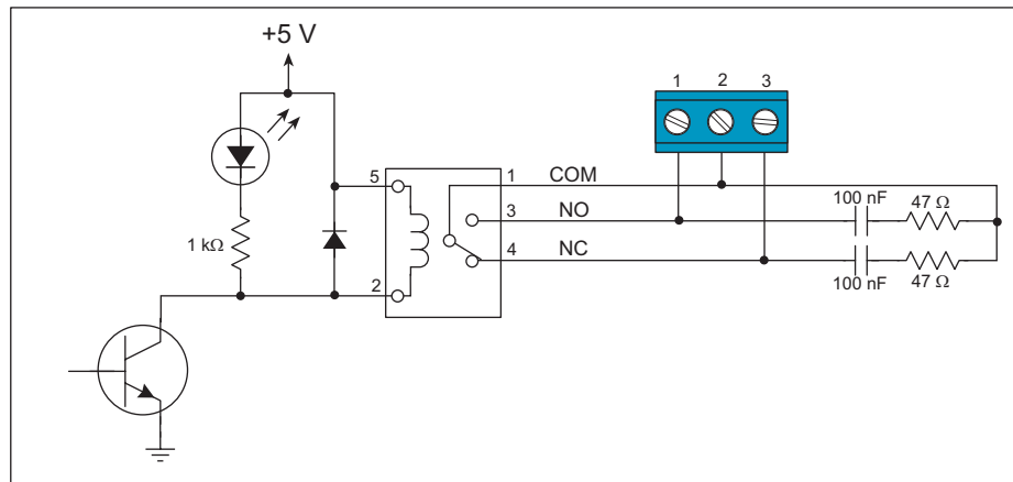
Figure 39. Relay Output Circuit
