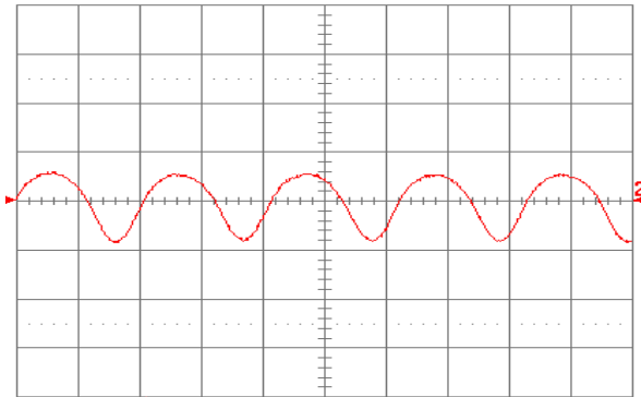
Figure 1.2V.21. Input reflected ripple current, i_c (100 mA/div.), measured at input terminals at full rated load current and V_{in} = 48 \text{ V} . Refer to Fig. 1.2V.20 for test setup. Time scale: 1 \mu\text{s}/\text{div} .
