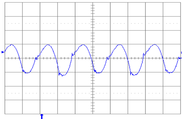
Figure 1.8V.19. Output voltage ripple (20mV/div.) at full rated load current into a resistive load with C_o = 10 \mu\text{F} tantalum + 1 \mu\text{F} ceramic and V_{in} = 48 \text{ V} . Time scale: 1 \mu\text{s}/\text{div} .
