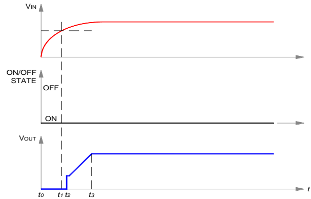
Figure 5. Start-up scenario #1.
