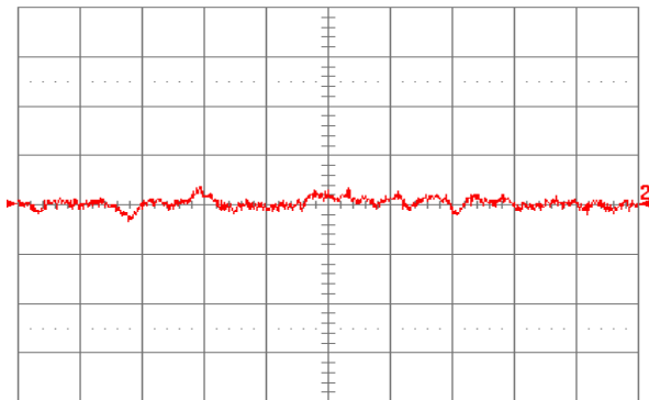
Figure 1.0V.22. Input reflected ripple current, i_s (10 mA/div.), measured through 10 \mu\text{H} at the source at full rated load current and V_{in} = 48 \text{ V} . Refer to Fig. 1.0V.20 for test setup. Time scale: 1 \mu\text{s}/\text{div} .
