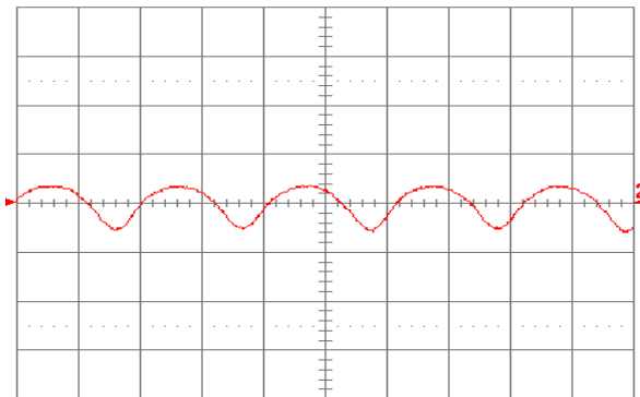
Figure 1.0V.21. Input reflected ripple current, i_c (100 mA/div.), measured at input terminals at full rated load current and V_{in} = 48 \text{ V} . Refer to Fig. 1.0V.20 for test setup. Time scale: 1 \mu\text{s}/\text{div} .
