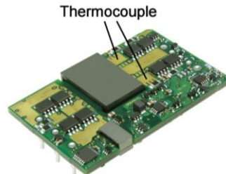
Figure 8. Location of the thermocouple for thermal testing.
