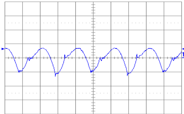
Figure 1.2V.19. Output voltage ripple (20 mV/div.) at full rated load current into a resistive load with C_o = 10 \mu\text{F} tantalum + 1 \mu\text{F} ceramic and V_{in} = 48 \text{ V} . Time scale: 1 \mu\text{s}/\text{div} .
