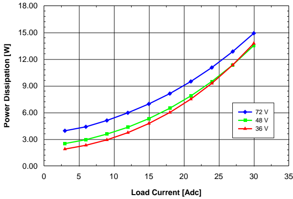
Figure 3.3V.13. Power dissipation vs. load current and input voltage for QME48T40033 converter mounted horizontally with air flowing from pin 1 to pin 3 at a rate of 300 LFM (1.5 m/s) and T_a = 25\text{ }^\circ\text{C} .
