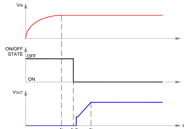
Figure 6. Startup scenario #2.
