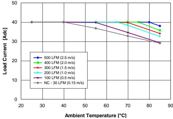
Figure 1.5V.9. Available load current vs. ambient air temperature and airflow rates for QME48T40015 converter with G height pins mounted vertically with air flowing from pin 1 to pin 3, MOSFET temperature \leq 120\text{ }^{\circ}\text{C} , V_{in} = 48\text{ V} .
