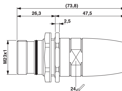
Dimensional drawing
