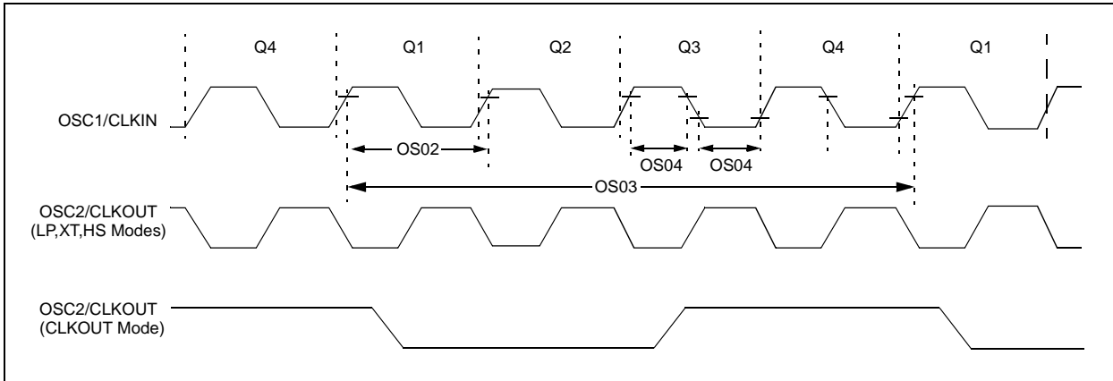
FIGURE 25-3: CLOCK TIMING
