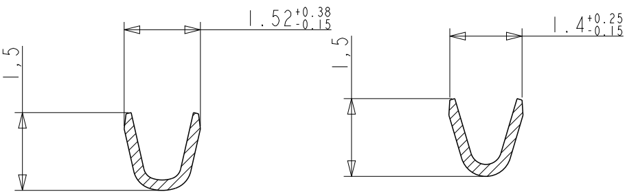
SECTION A-A SECTION B-B CROSS SECTIONS FOR CT #24-28
