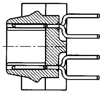
SECT "A"-"A"
