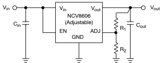
Figure 4. NCV8606 Typical Application Circuit for Adjustable Version ( 1.25\text{ V} < V_{out} \leq 5.0\text{ V} )
