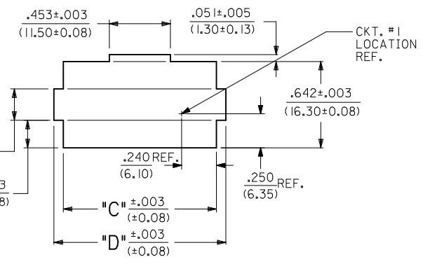
RECOMMENDED CUT-OUT FOR .063/(1.60) MAX. .038/(0.97) MIN. THICK PANEL (6-24 CKT'S.) SCALE: 2X
