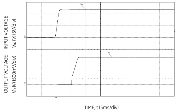
Figure 12. Typical Start-up Using Input Voltage (VIN = 12V, Cext= 22μF, Io = Io,max).
