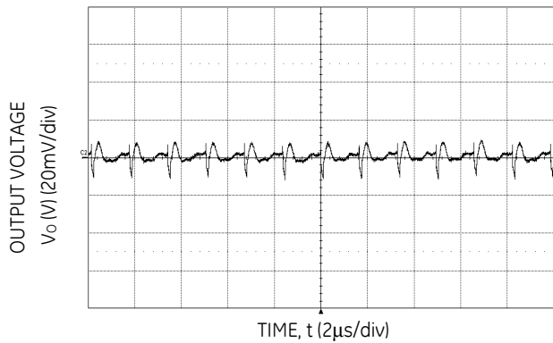
Figure 3. Typical output ripple and noise (VIN = 12V, Io = Io,max).
