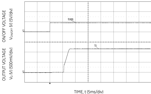
Figure 11. Typical Start-up Using On/Off Voltage (Io = Io,max, Vin=12V, Cext= 22μF).
