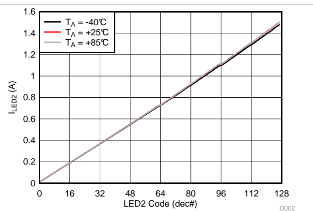
Figure 3. LED2 Flash Current vs Brightness Code
