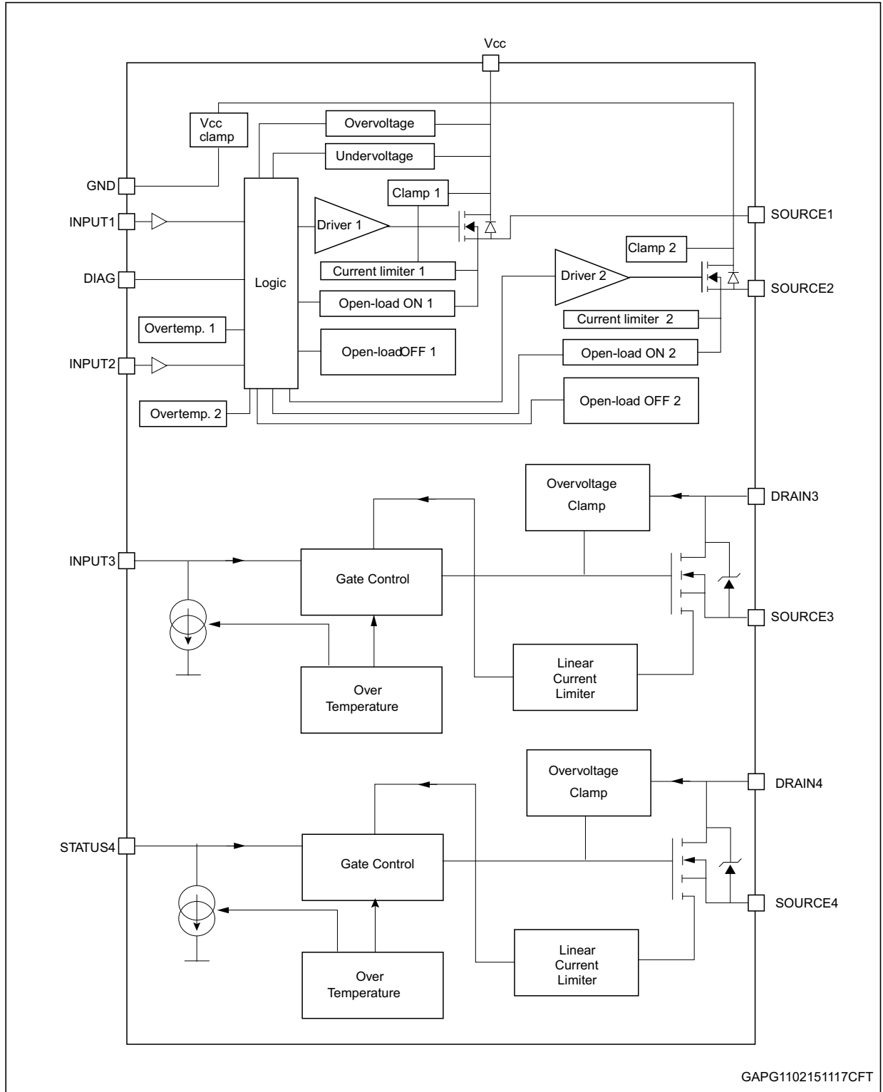
Figure 1. Block diagram
