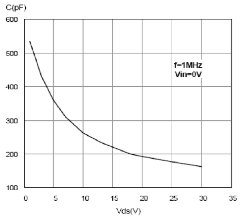
Figure 30. Capacitance variations
