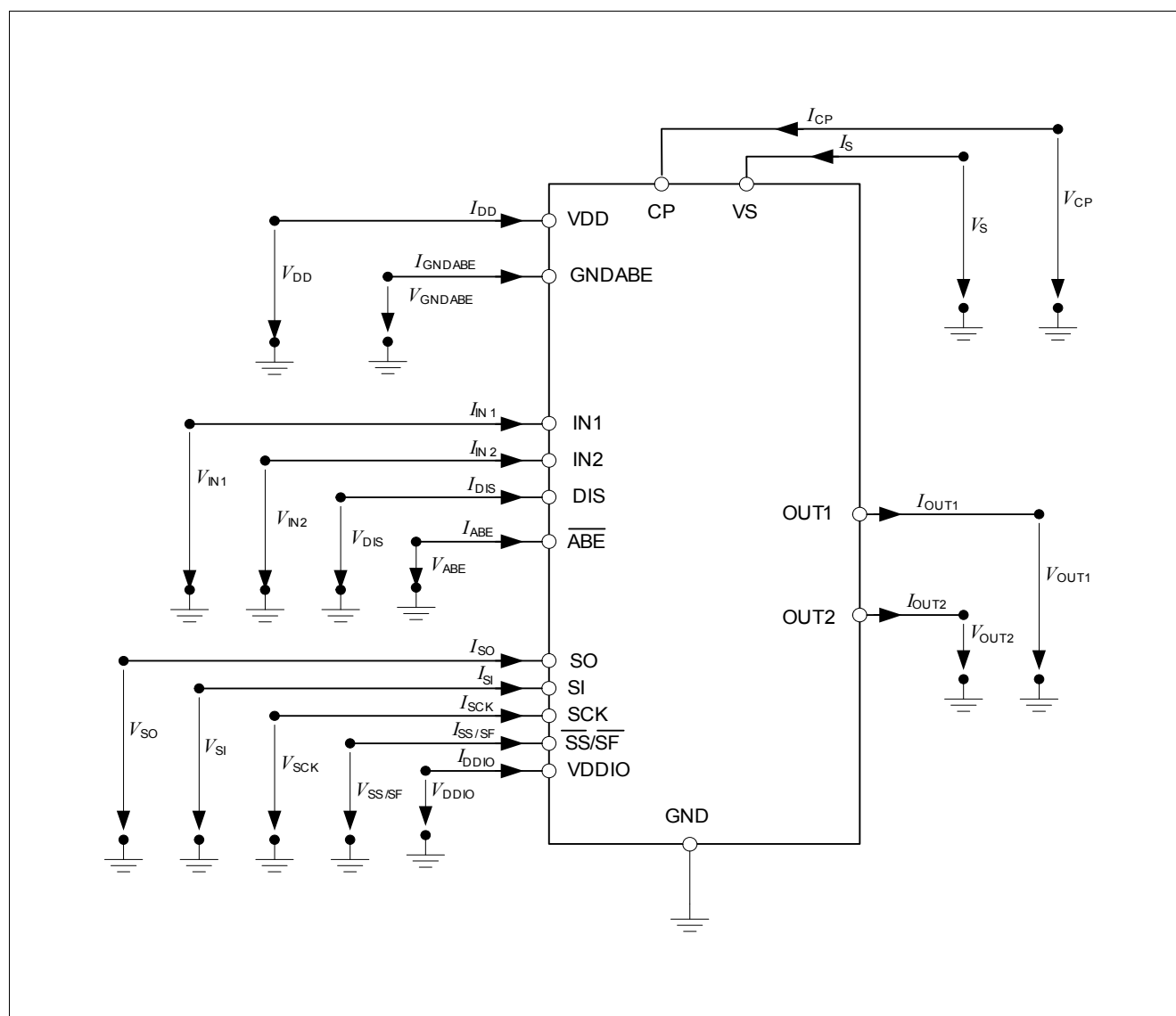
Figure 2 Terms TLE8209-2SA
