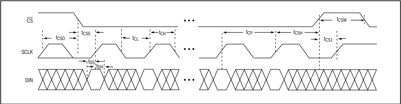
Figure 6. Detailed Serial-Interface Timing Diagram
