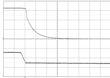
Shut-down enabled by disconnecting V_i at: T_{ref} = +25^{\circ}C , I_o = 10 A load, V_i = 53 V. Top trace: output voltage (1 V/div.). Bottom trace: input voltage (20 V/div.). Time scale: 0.1 ms/div..
