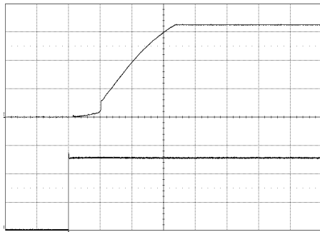
Start-up enabled by connecting V_i at: T_{ref} = +25^{\circ}C , I_o = 50 A resistive load, V_i = 53 V. Top trace: output voltage (1 V/div.). Bottom trace: input voltage (20 V/div.). Time scale: 5 ms/div..
