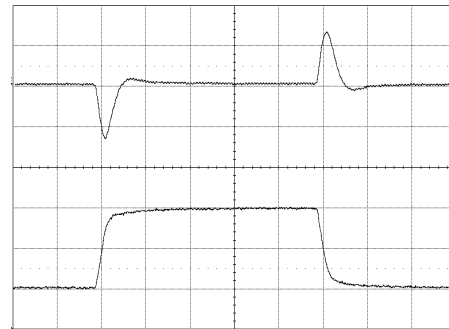
Output voltage response to load current step-change (12.5-47.5-12.5 A) at: T_{ref} = +25^{\circ}C , V_i = 53 V. Top trace: output voltage (200mV/div.). Bottom trace: load current (12.5 A/div.). Time scale: {0.1 ms/div..}
