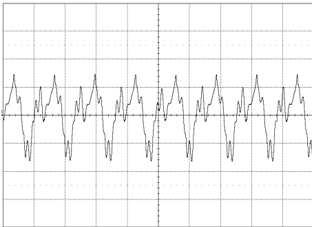
Output voltage ripple (20mV/div.) at: T_{ref} = +25^{\circ}C , I_o = 50 A resistive load, V_i = \{53 V}. Time scale: 5 \mu s/div. See the filter in the Output ripple and noise section (EMC Specification).
