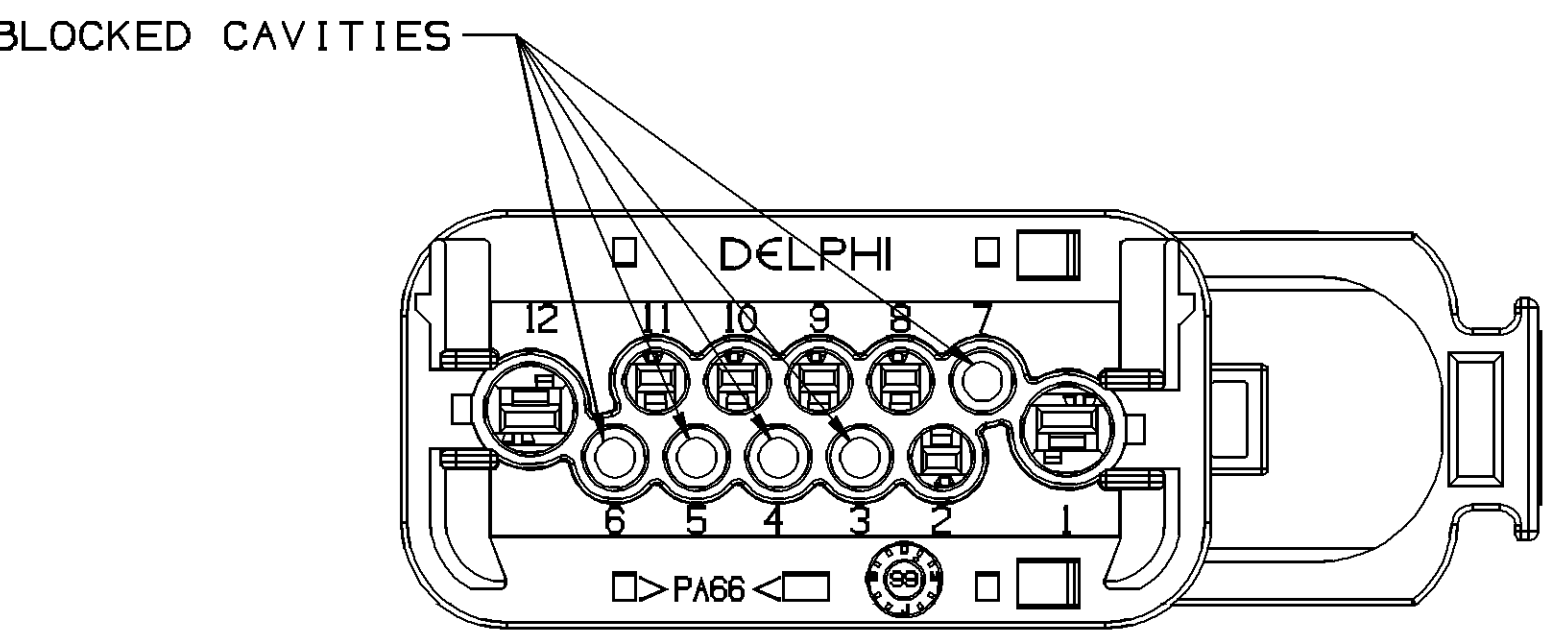
TYPE 203 SAME AS TYPE 201 EXCEPT AS SHOWN
