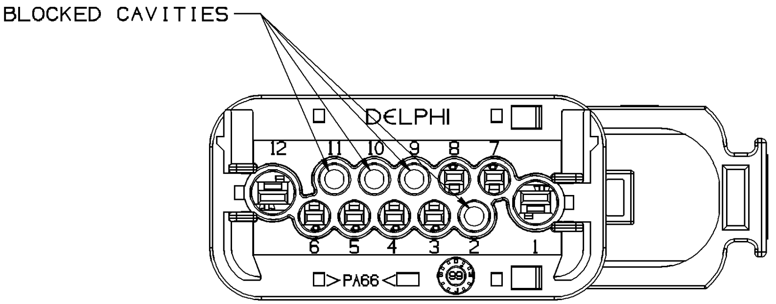
TYPE 204 SAME AS TYPE 201 EXCEPT AS SHOWN
