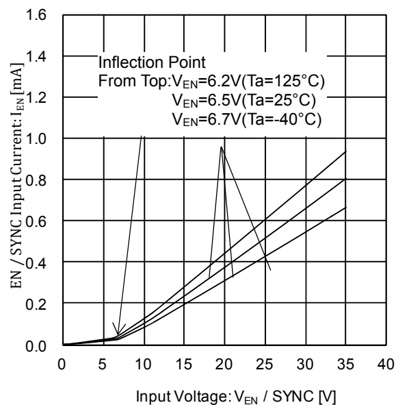
Figure 8. EN/SYNC Input Current vs Input Voltage
