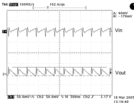
Figure 7. Ripple 150mA Torch, V_{in}=4.2V , V_{out}=3.1V . C_{in}=4.7\mu F , C_{FC}=0.47\mu F , C_{out}=2.2\mu F .
