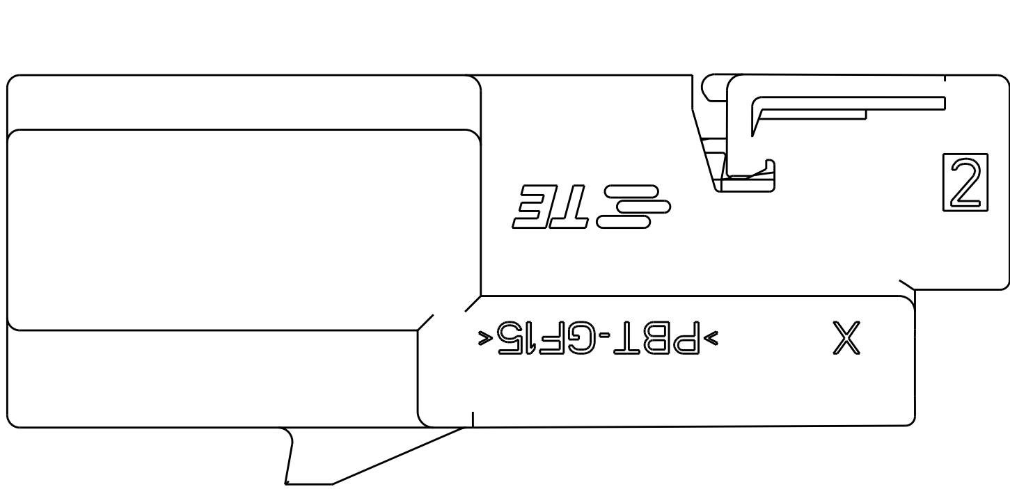
2138558-1 ASSEMBLED VIEW
