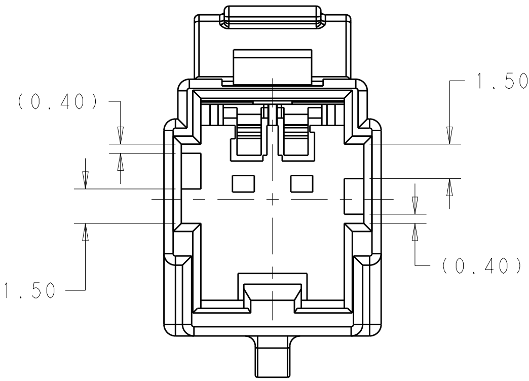
KEYING OPTION B WITH RETAINER CLIP LOCK 2138558-2
