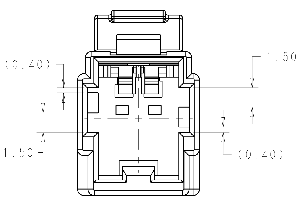
KEYING OPTION B WITHOUT RETAINER CLIP LOCK 2138558-4
