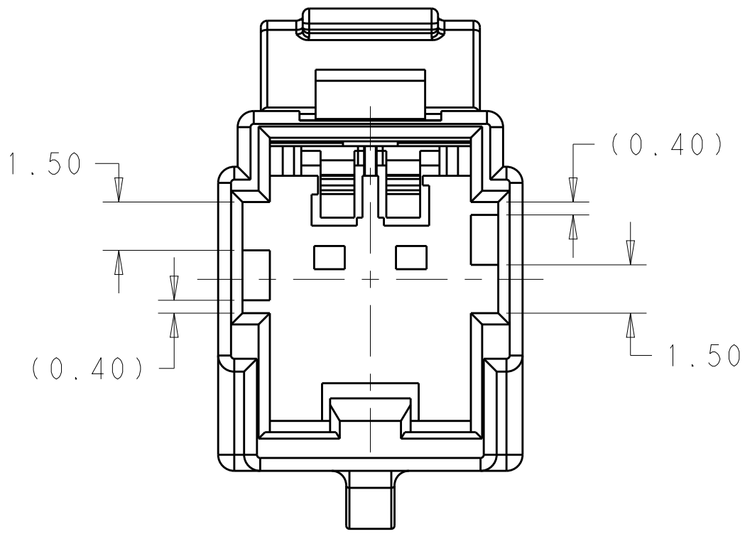
KEYING OPTION A WITH RETAINER CLIP LOCK 2138558-1
