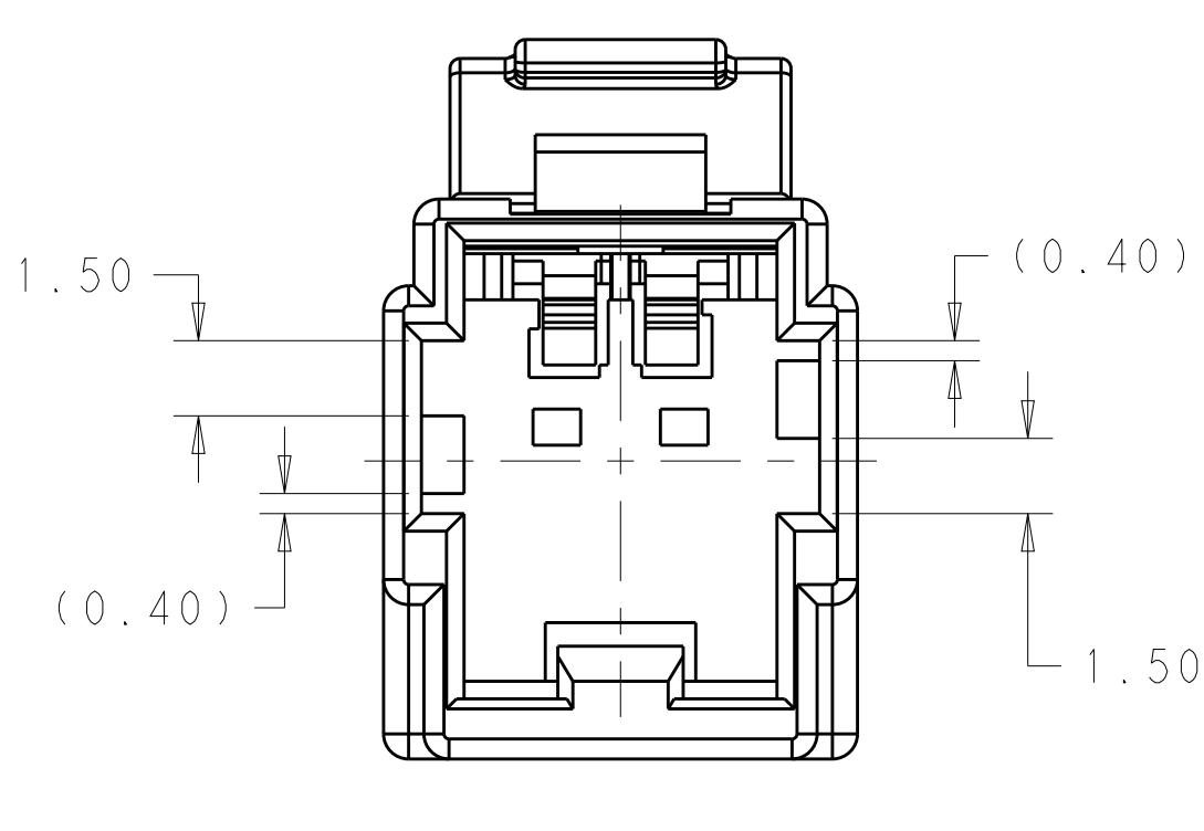
KEYING OPTION A WITHOUT RETAINER CLIP LOCK 2138558-3
