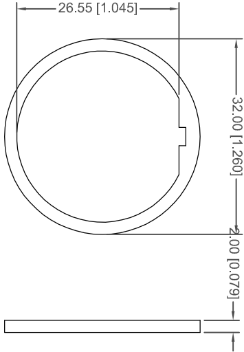
O-RING
