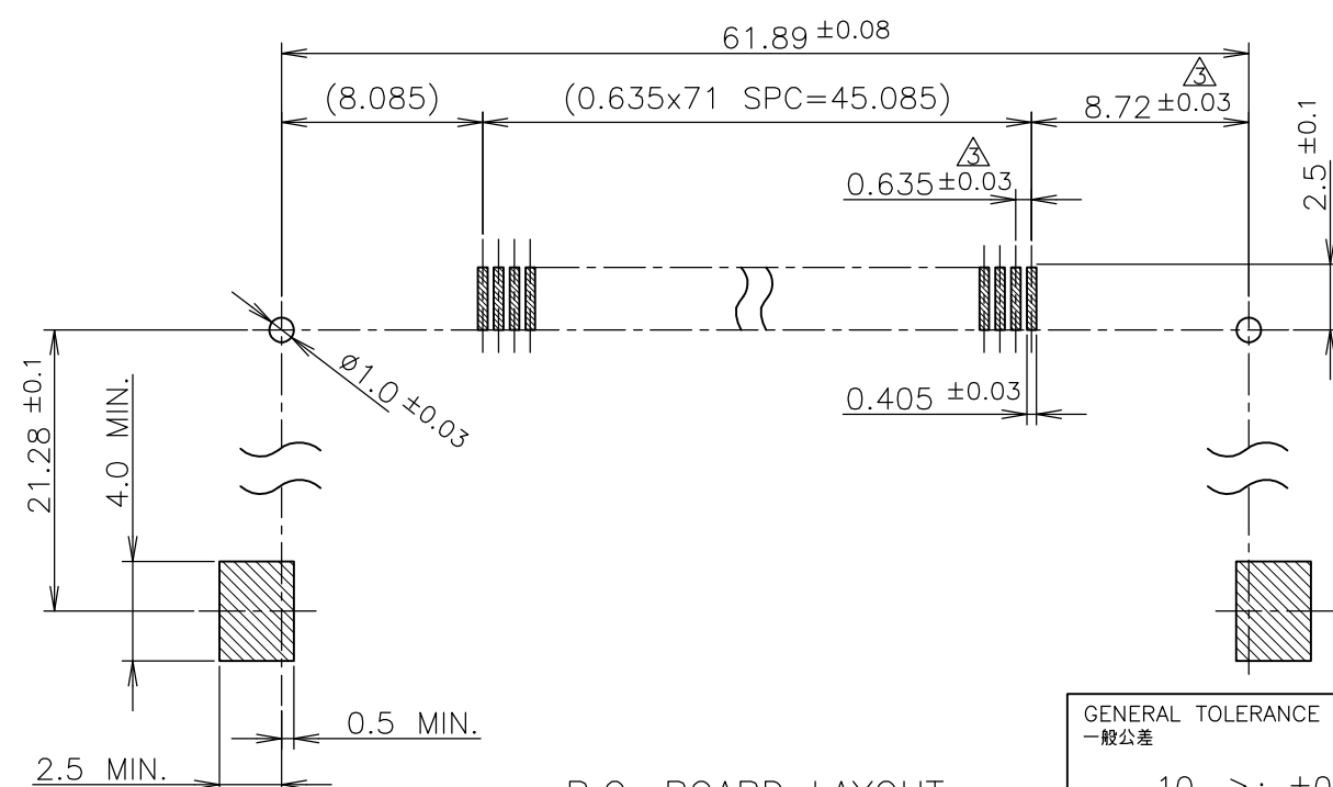
P.C. BOARD LAYOUT (CONNECTOR MOUNT SIDE)
