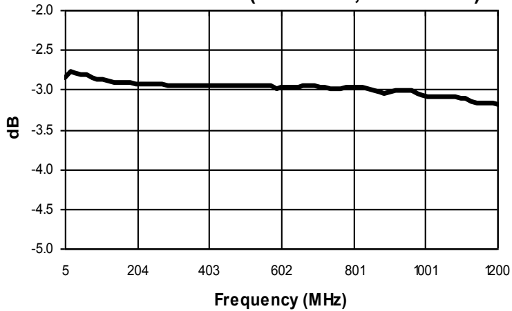
Amplitude Balance
