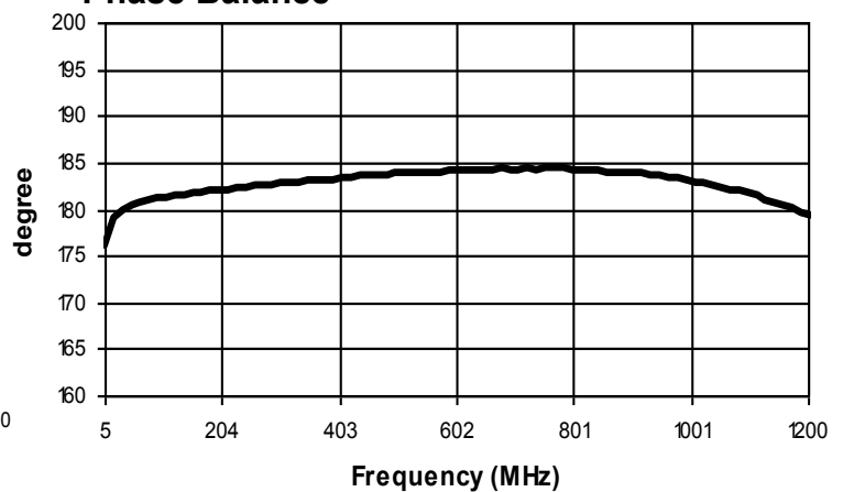
Phase Balance
