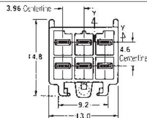
Section Y-Y
