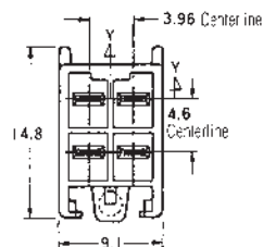
Section Y-Y
