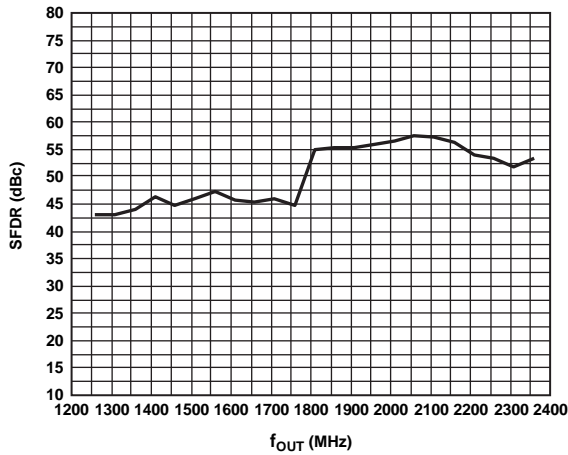
Figure 108. SFDR in Mix-Mode vs. f_{OUT} at 2.4 GSPS
