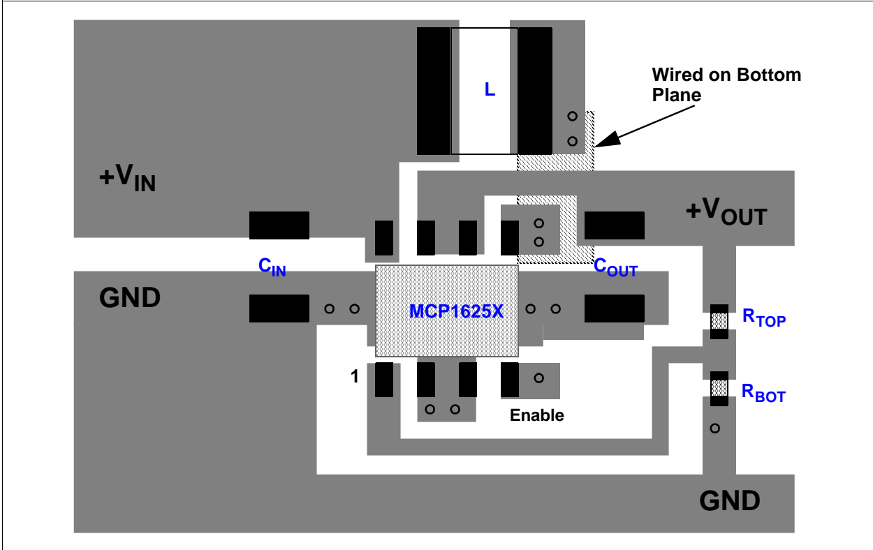
FIGURE 5-2: MCP16251/2 TDFN-8 Recommended Layout.
