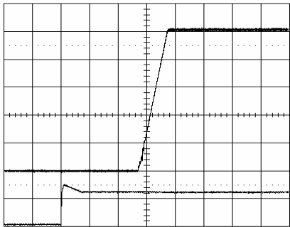
Start-up enabled by connecting V_I at: T_{P1} = +25^{\circ}\text{C} , V_I = 12\text{ V} , I_O = 40\text{ A} resistive load and 10\text{ mF} . Top trace: output voltage (0.2 V/div.). Bottom trace: input voltage (10 V/div.). Time scale: (10 ms/div.).
