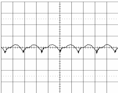
Output voltage ripple at: T_{P1} = +25^{\circ}\text{C} , V_I = 12\text{ V} , I_O = 40\text{ A} resistive load. Trace: output voltage (20 mV/div.). Time scale: (2 \mu\text{s} /div.).
