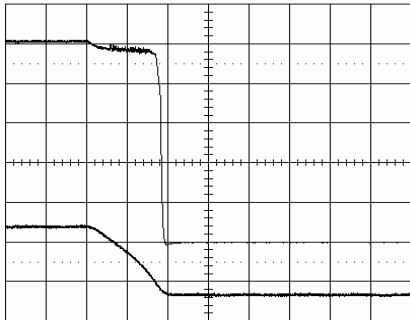
Shut-down enabled by disconnecting V_I at: T_{P1} = +25^{\circ}\text{C} , V_I = 12\text{ V} , I_O = 40\text{ A} resistive load. Top trace: output voltage (0.2 V/div.). Bottom trace: input voltage (5 V/div.). Time scale: (0.5 ms/div.).
