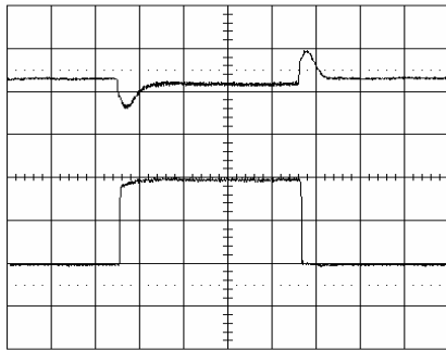
Output voltage response to load current step-change (10-30-10 A) at: T_{P1} = +25^{\circ}\text{C} , V_I = 12\text{ V} , C_O = 10\text{ mF} . Top trace: output voltage (50 mV/div.). Bottom trace: load current (10 A/div.). Time scale: (0.5 ms/div.).
