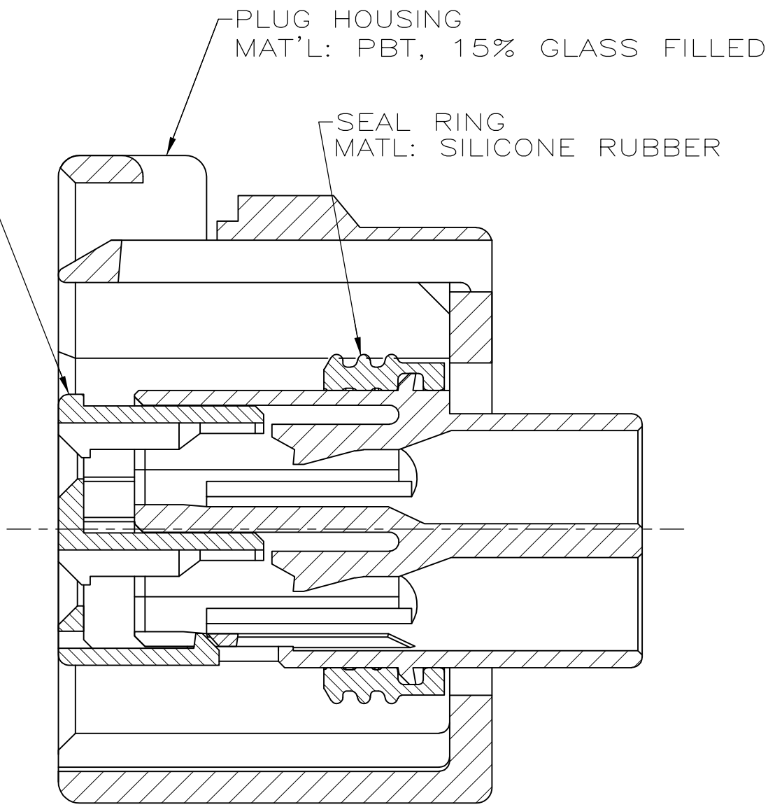
SECTION Z-Z SCALE 4:1
