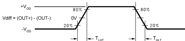
Figure 7. LVDS Output Transition Times
