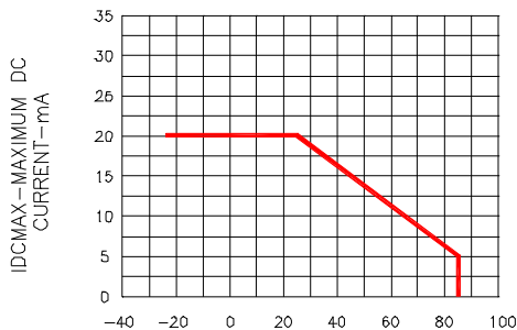
TA - AMBIENT TEMPERATURE °C
