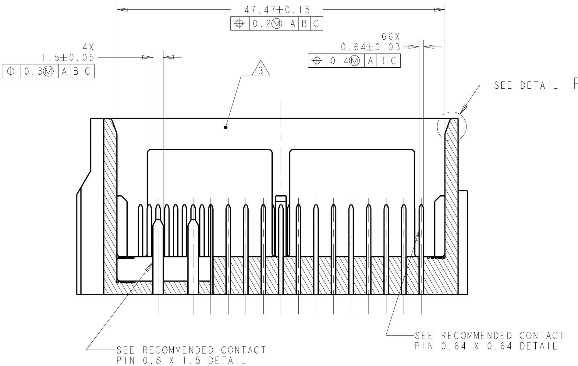
SECTION B-B
