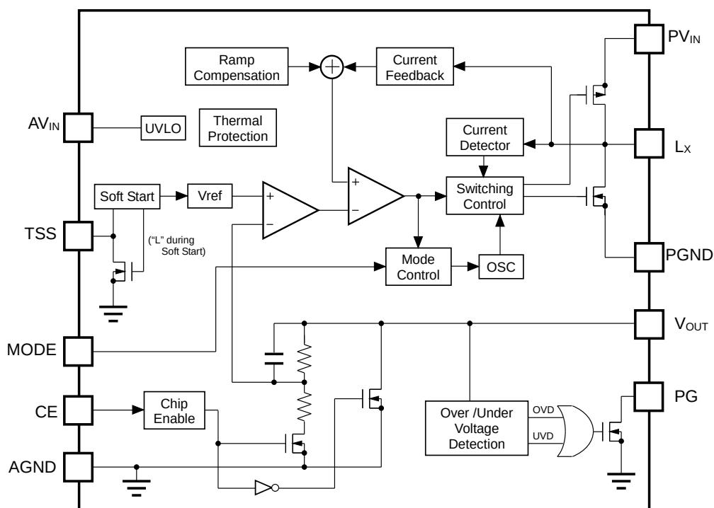
RP506Kxx1B/E Block Diagram
