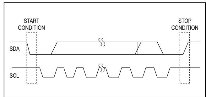
Figure 4. START/STOP Conditions
