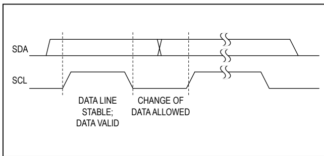
Figure 3. Bit Transfer
