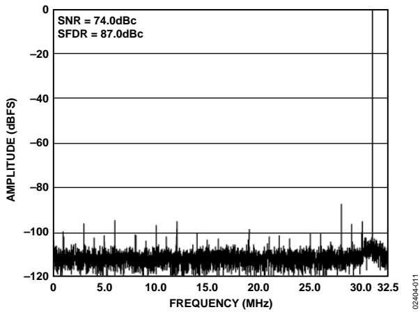
Figure 11. Single-Tone FFT, f_{IN} = 31 MHz
