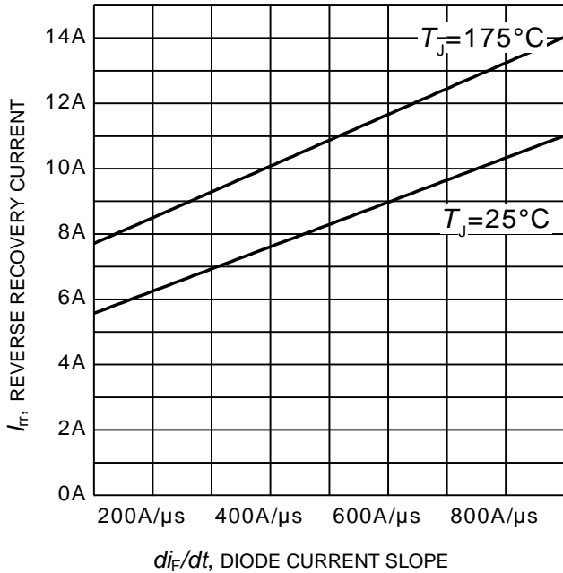
di_F/dt , DIODE CURRENT SLOPE Figure 25. Typical reverse recovery current as a function of diode current slope ( V_R = 400V , I_F = 10A , Dynamic test circuit in Figure E)
