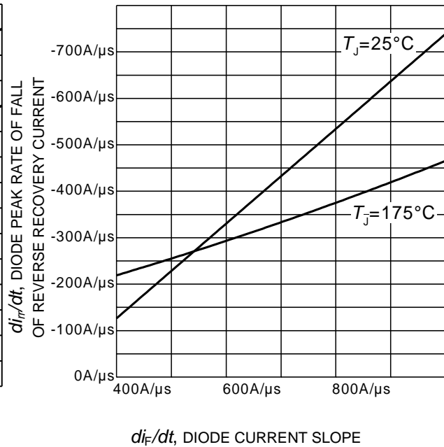
di_F/dt , DIODE CURRENT SLOPE Figure 26. Typical diode peak rate of fall of reverse recovery current as a function of diode current slope ( V_R = 400V , I_F = 10A , Dynamic test circuit in Figure E)
