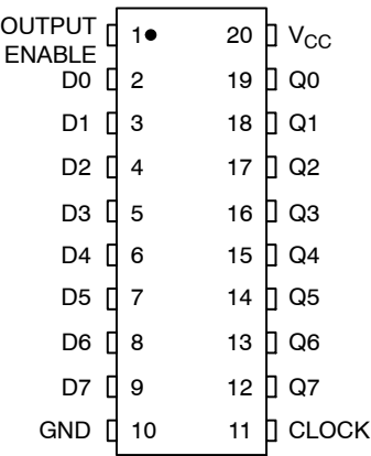
Figure 1. Pin Assignment
