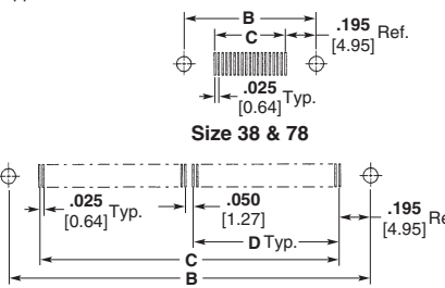
Size 120, 152 & 200 Recommended PCB Footprint Pattern
