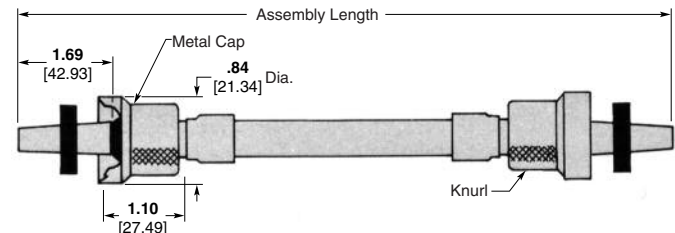
Part Number 861814
