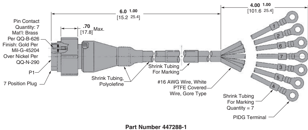
Part Number 447288-1
