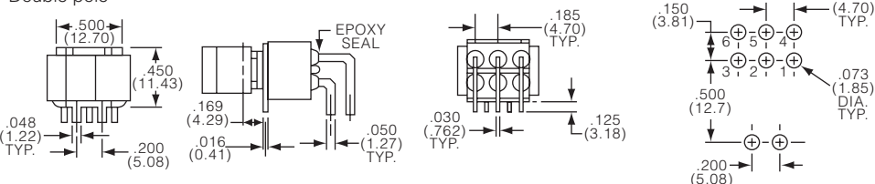
Double pole
