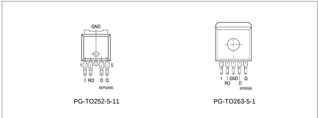
Figure 2 Pin Assignment
