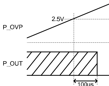
Figure 30. Timing Chart
