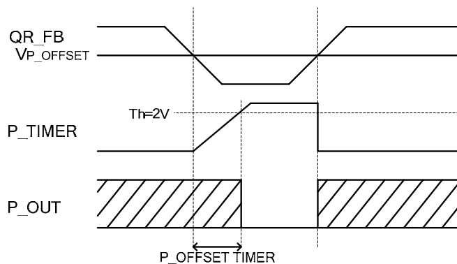
Figure 37. Timing Chart
