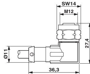
Dimensional drawing
