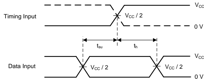
Figure 12. Voltage Waveforms: Setup and Hold Times
