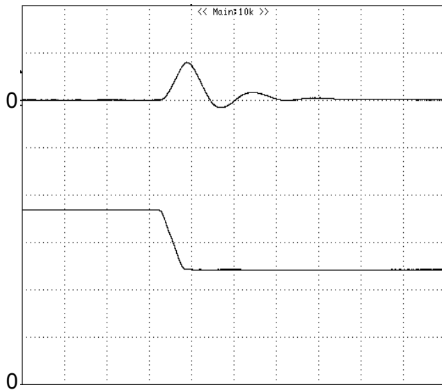
Figure 8: Output voltage response to step-change in load current (75%-50% of I_o , max; di/dt = 0.1A/\mu s ). Load cap: 10\mu F tantalum capacitor and 1\mu F ceramic capacitor. Top Trace: V_{out} (100mV/div, 50us/div), Bottom Trace: I_{out} (2A/div). Scope measurement should be made using a BNC cable (length shorter than 20 inches). Position the load between 51 mm to 76 mm (2 inches to 3 inches) from the module
