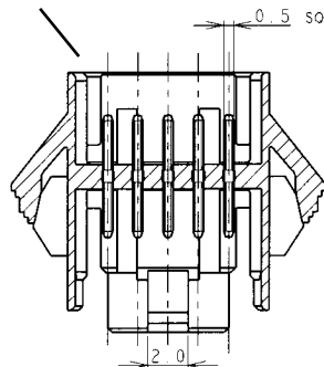
SECT B-B
